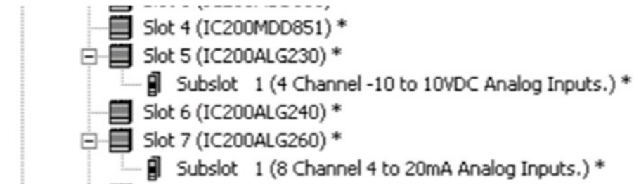
Figure 72: Analog Modules Showing Configuration Mismatch Cleared
