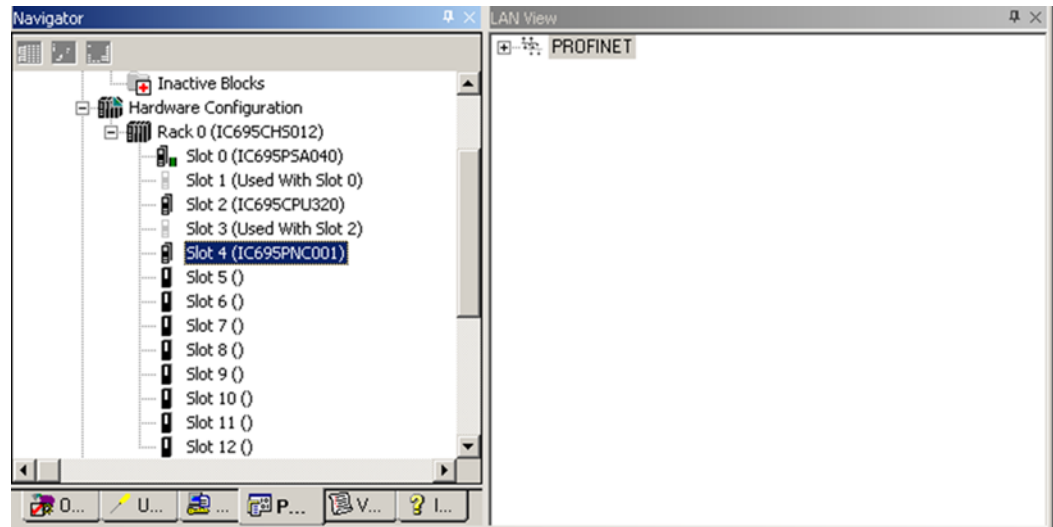
Figure 48: Configuring the PROFINET LAN
