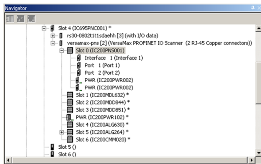
Figure 69: VersaMax PNS Rack showing Power Supply Located between I/O Modules
