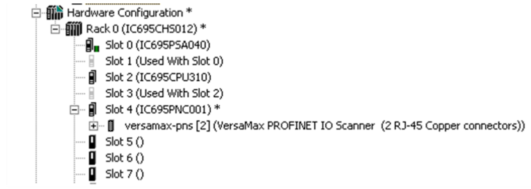
Figure 54: PNS Attached to PNC001 in PAC MACHINE EDITION Navigator
