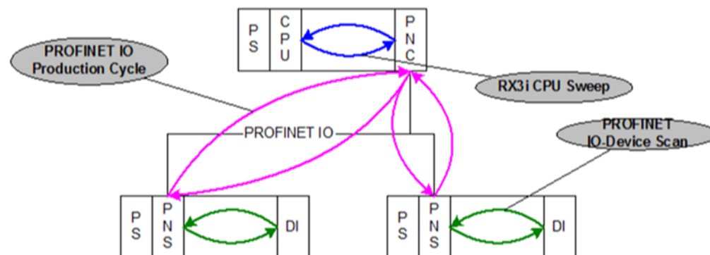
Figure 92: Diagram of Multiple Asynchronous I/O Scans
