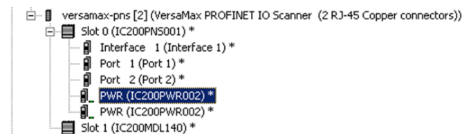
Figure 65: Power Supplies Displayed in PNS Rack
