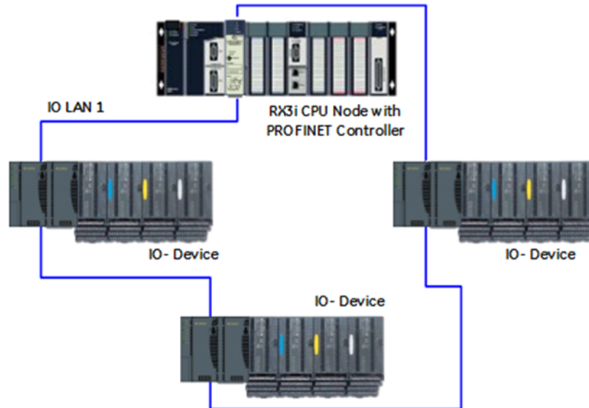
Figure 100: Ring Topology with One Controller
