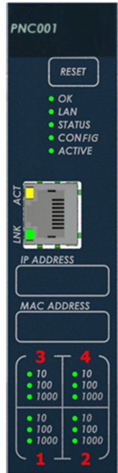
Figure 32: PNC001-Bxxx Front View showing LEDs
