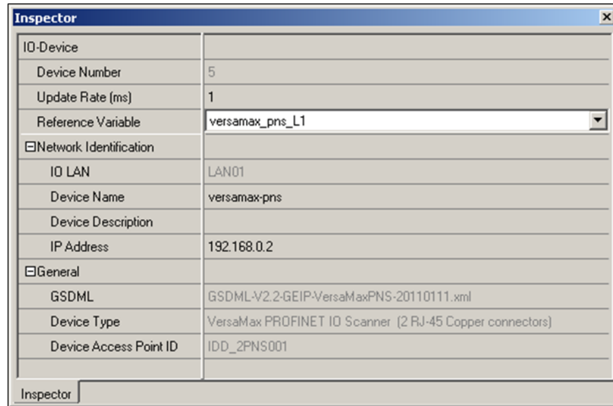
Figure 85: Assigning Reference Variable to IO-Device
