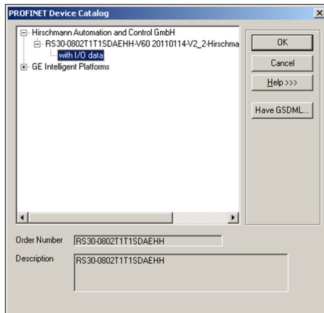
Figure 73: Selecting Third-Party Modules for Addition to LAN
