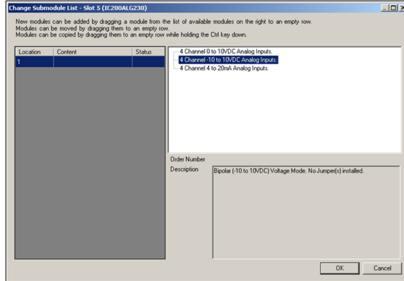
Figure 71: Selecting the Sub-Module Configuration with Jumper Settings Declared
