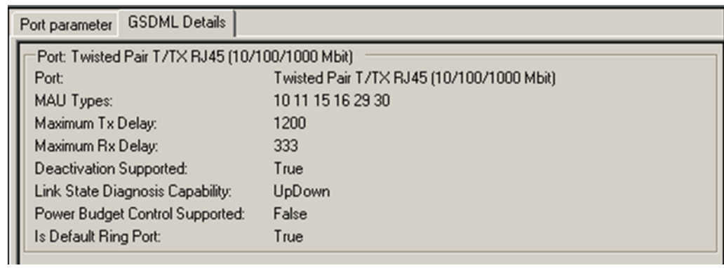
Figure 82: Display of GSDML for Third-Party I/O Device
