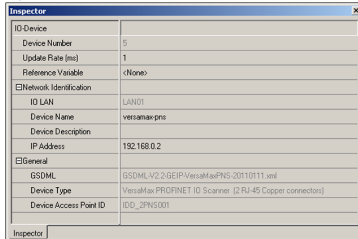
Figure 83: Inspector View of IO-Device Properties
