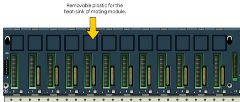
Figure 19: RX3i Backplane showing Removable Plastic Knockout
