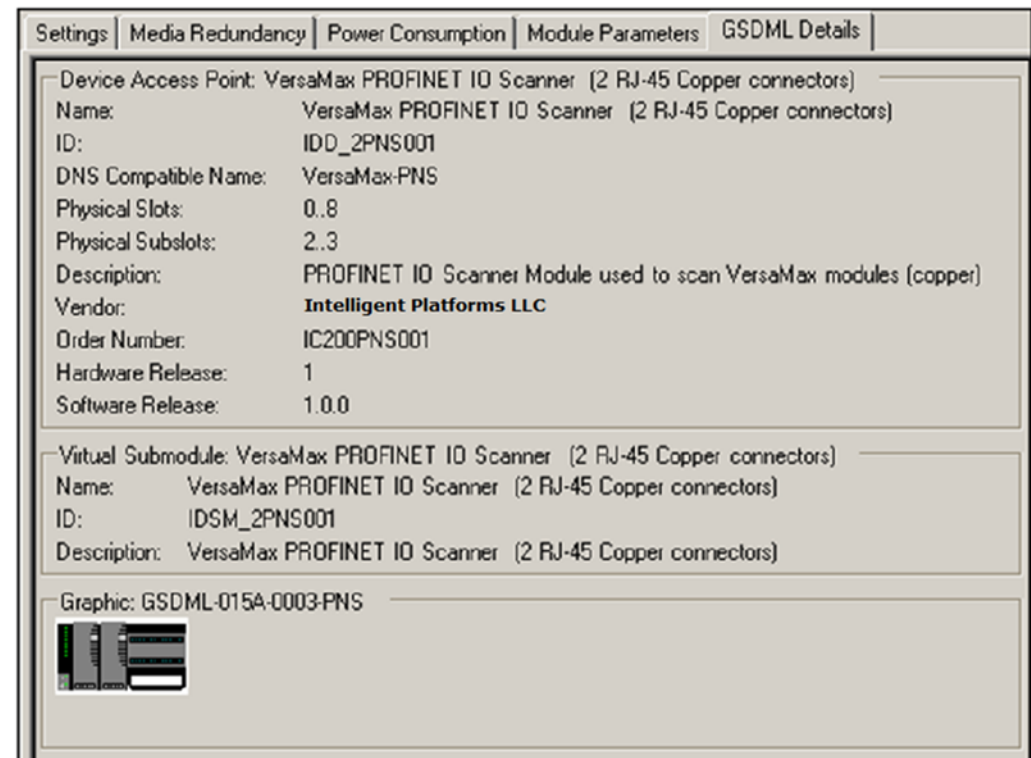
Figure 61: PNS Parameters GSDML Details Tab
