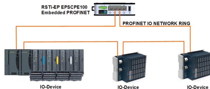
Figure 18: RX3i System with one PROFINET Controller and PROFINET IO Network MRP
