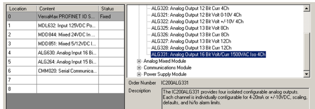
Figure 67: Select VersaMax Module from Available List
