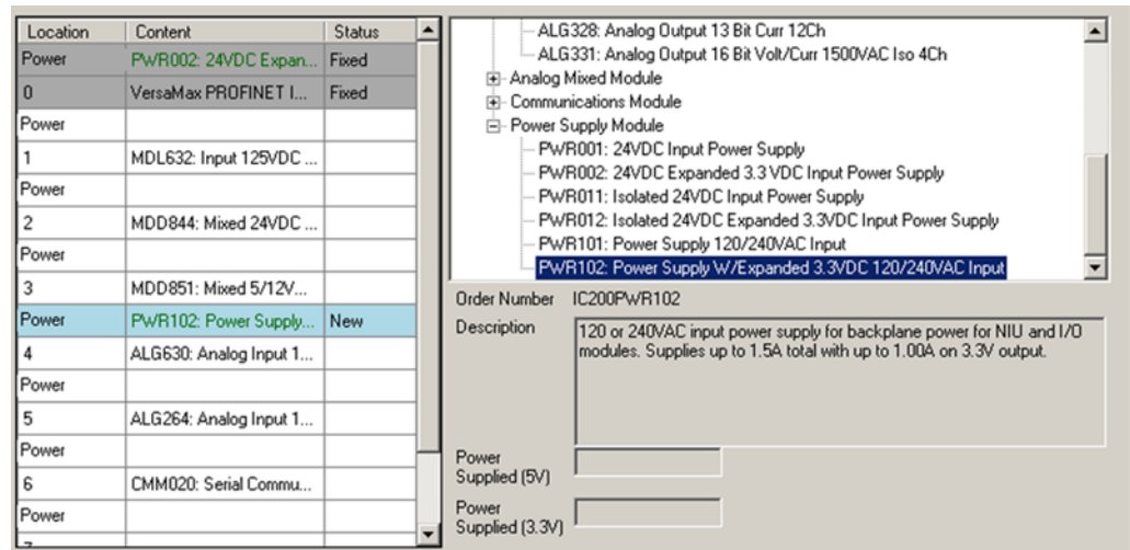
Figure 68: Adding Power Supplies between Modules in PNS Rack
