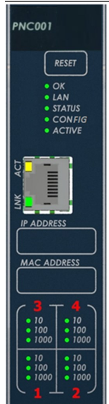
Figure 1: IC695PNC001-Bxxx Front View
