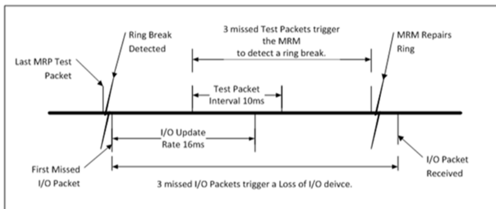
Figure 99: Timeline for Successful MRP Ring Repair at 16ms I/O Update Rate
