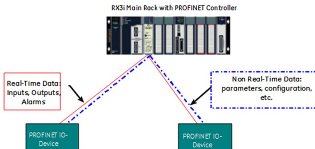
Figure 91: Real-Time and Non-Real-Time Data Communications
