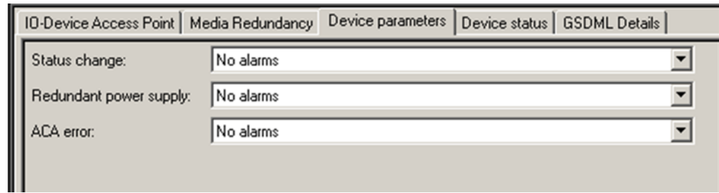
Figure 79: Third-Party I/O: Additional Parameter Settings (Product Dependent)
